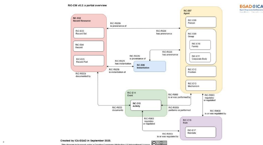
Fig. 1. Overview of RiC-CM main entities
